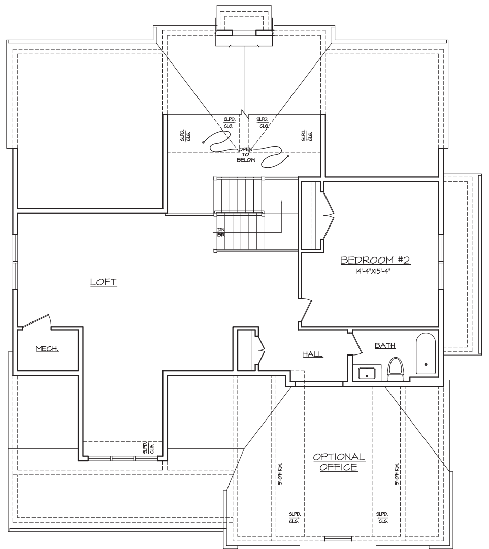
SECOND FLOOR | 976 SF +/-
