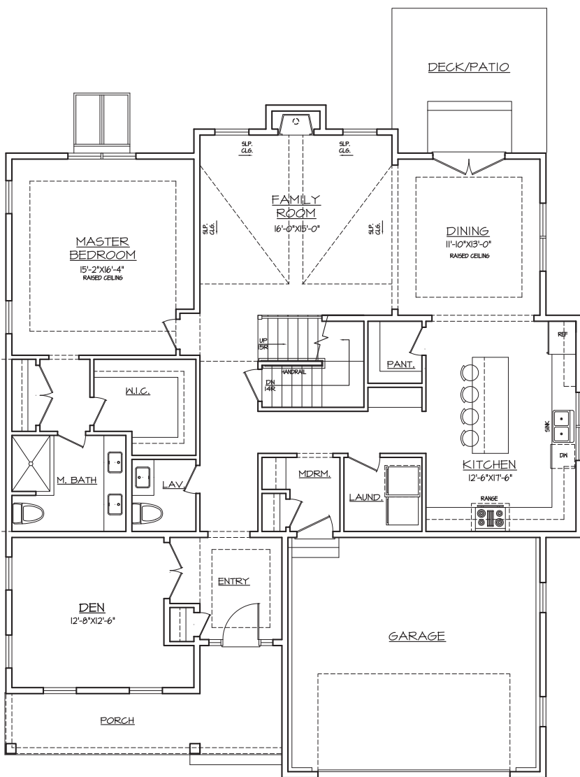
FIRST FLOOR | 1,806 SF +/-
